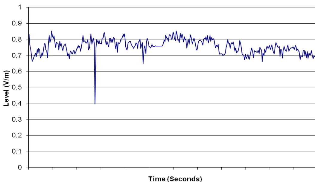
Electric field strengths recorded over 6 min period using 18 GHz probe at point of max NIR:
